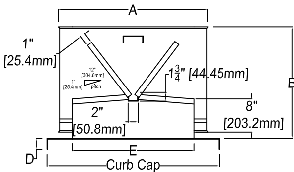
Model I-200-C curb cap style (shown)
